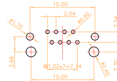
PC Board Layout Component Side Shown PC Board Thickness=1.6mm Tolerance±0.05
